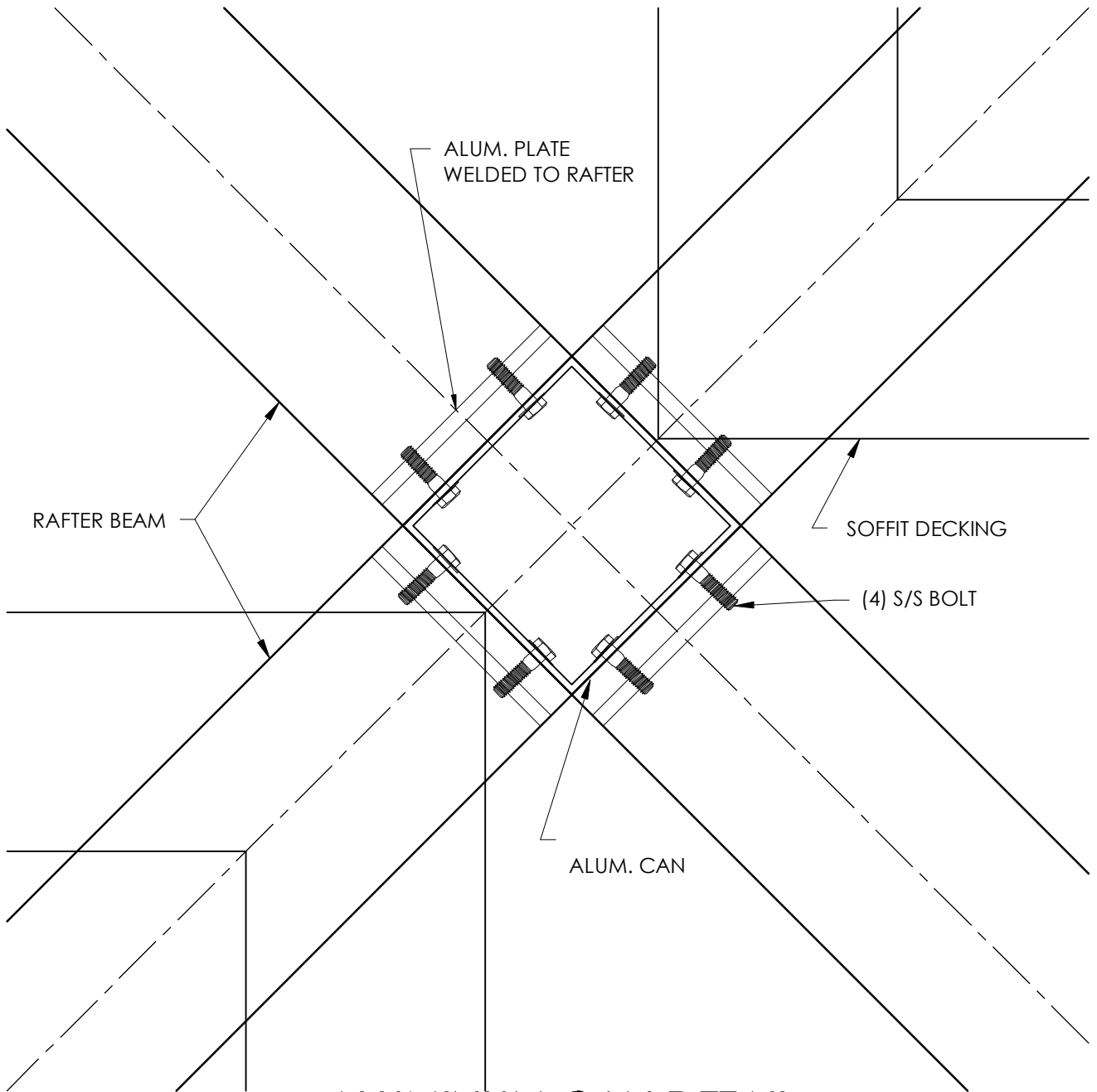
ALUMINUM CAN DETAIL PLAN VIEW
