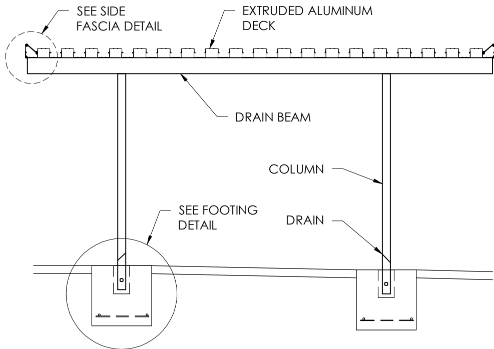
SINGLE CAR CARPORT SECTION
